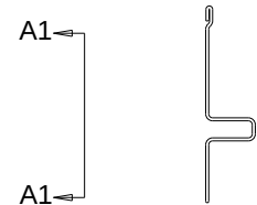
LEFT SIDE RAFTER HOLE PUNCH (A - A)
